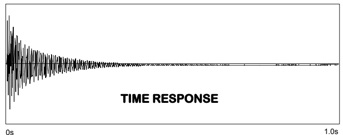
Figure 2 – Time Response Output for 800 Hz Bandwidth
