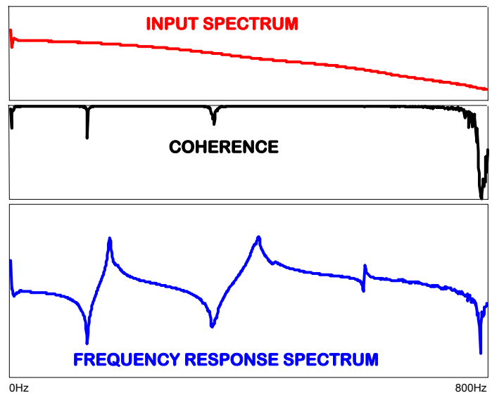
Figure 1 – Input Spectrum, Coherence and Frequency Response Function over an 800 Hz Bandwidth
