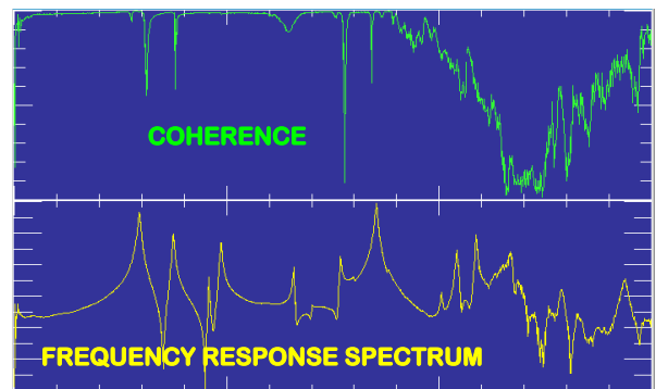
Figure 5 – FRF/Coherence for POD Measurement
