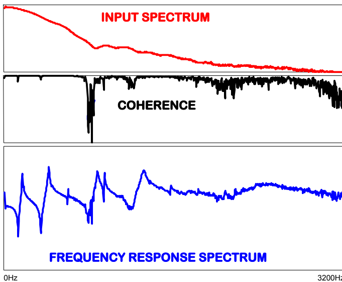
Figure 4 – Input Spectrum, Coherence and Frequency Response Function over a 3200 Hz Bandwidth
