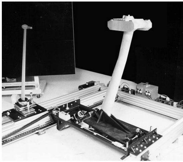
Figure 6. View of the Target Positioning System with Free-Space Calibration Disk (Left) and Complex Target Simulator (Right) Attached to Low-RCS Pylons.
