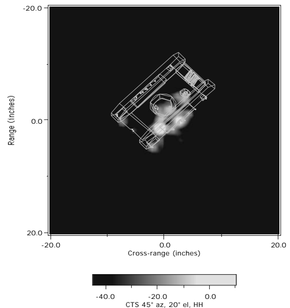
Figure 7. An Example of an X-band ISAR Image of Complex Target Simulator with line drawing overlay ( 45^\circ az, 20^\circ el, HH).
