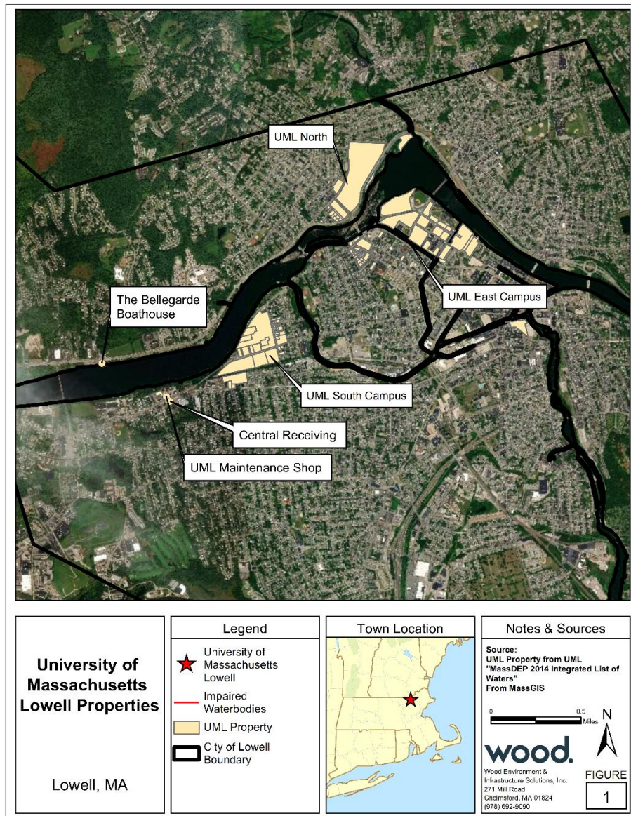
Figure 1: UML Properties
