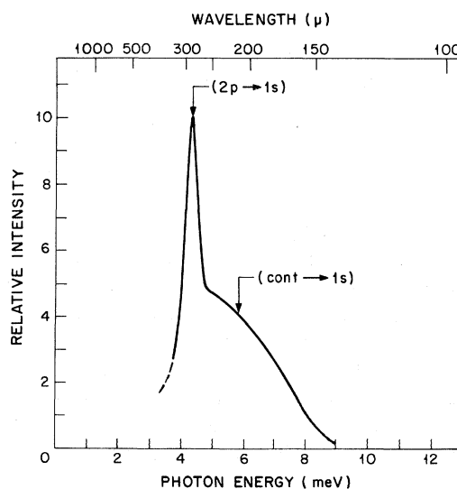
FIG. 1. Radiation spectrum of impact-ionized GaAs sample at 4.2^\circ\text{K} biased with 260- \mu\text{sec} -long, 100-mA pulses at a 1-kHz repetition rate.
