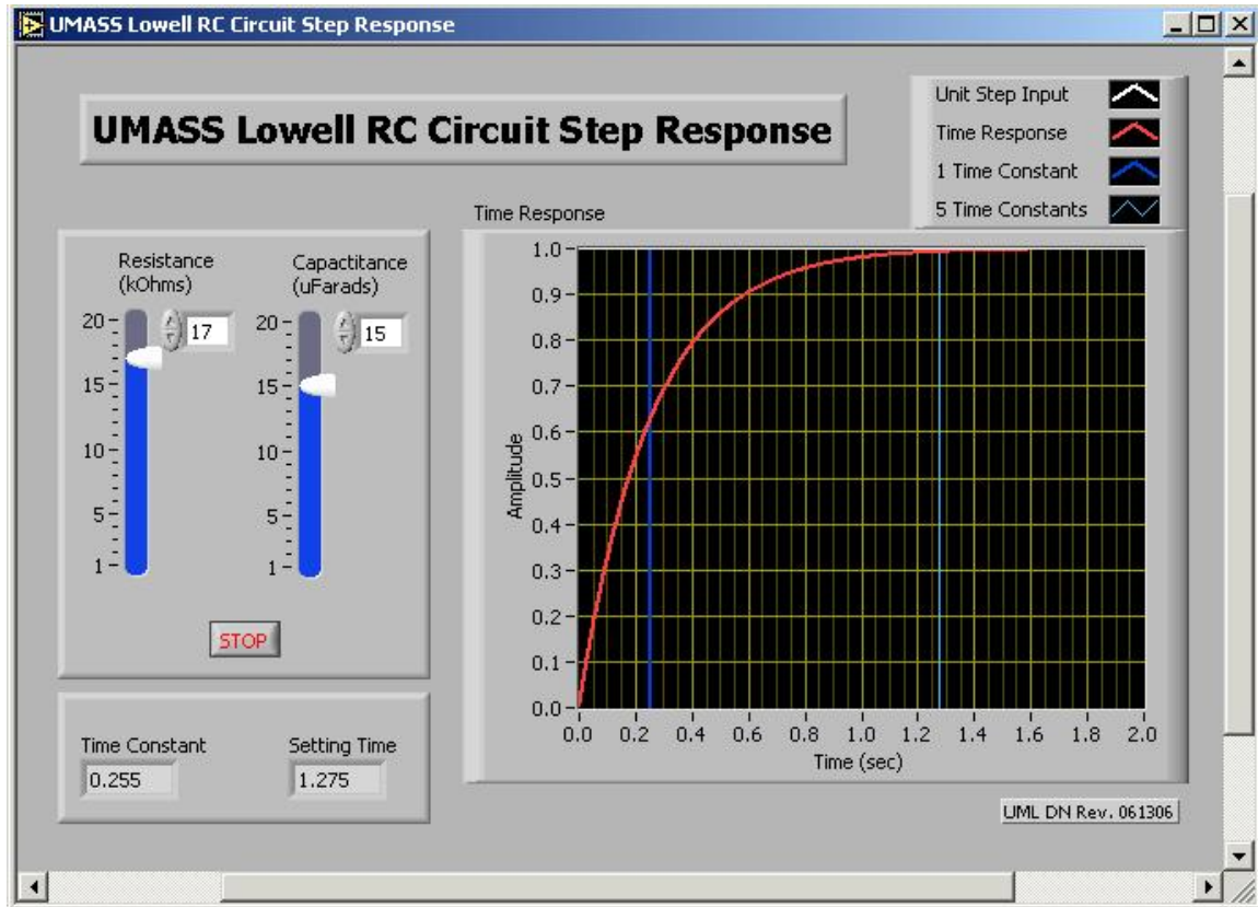
Figure 1. RC Step LabVIEW GUI Front Panel
