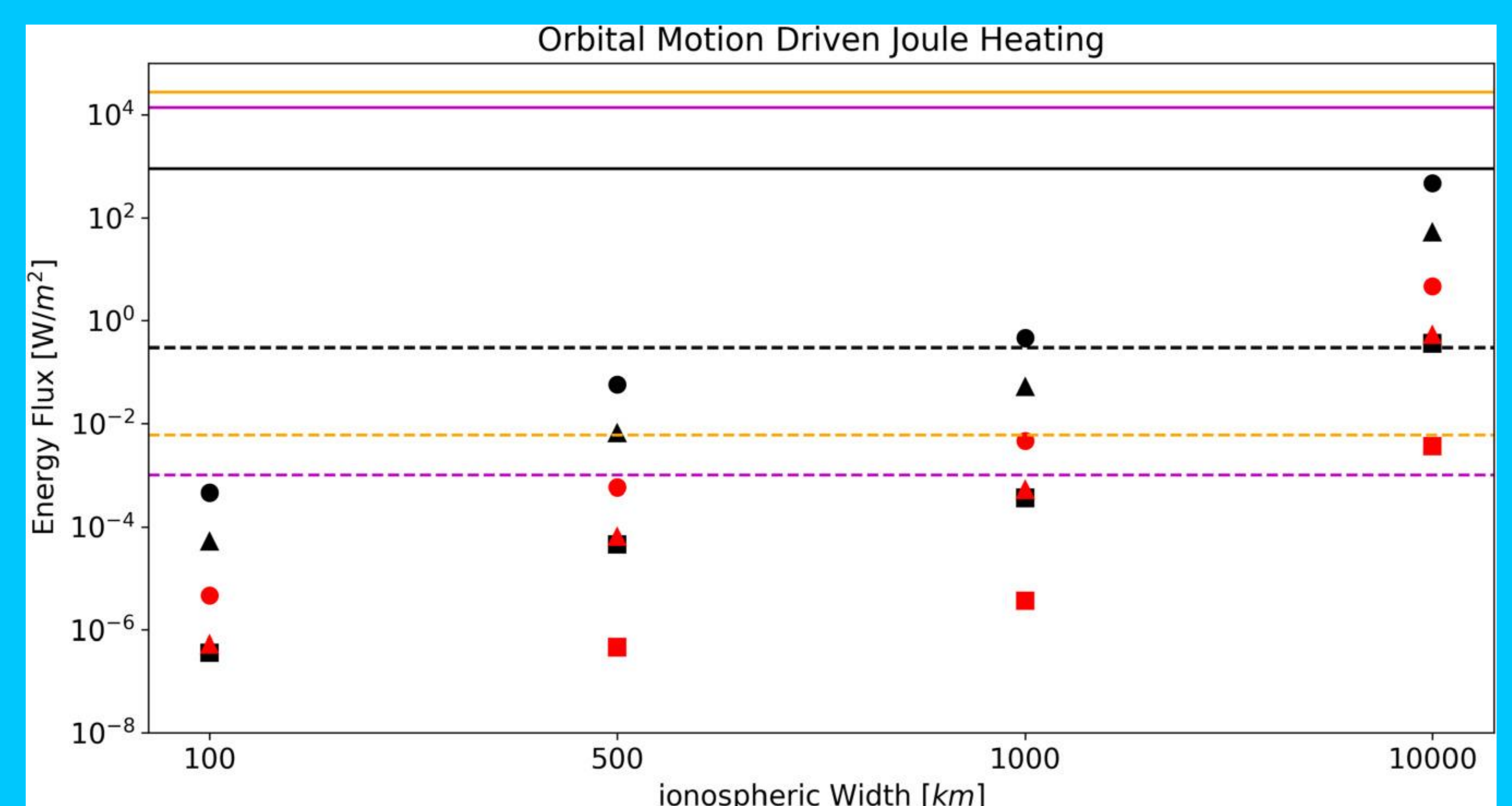
Figure 4. Maximum Joule Heating energy flux in [\text{W/m}^2] as a function of ionospheric width using the maximum value of dB/dt for the synthetic data sets of Trappist-1e (circles), the solar case at 0.05 AU (triangles), and the solar case at 0.1 AU (squares). The red markers represent the energy flux using \sigma = 0.1 [\text{S/m}] , while the black markers represent the energy flux using \sigma = 10 [\text{S/m}] . Also shown are the reference energy fluxes of the stellar/solar constant radiation (solid lines) and EUV radiation (dashed lines) for the orbits of Trappist-1e (black), 0.05 au (orange), and 0.1 au (magenta).
