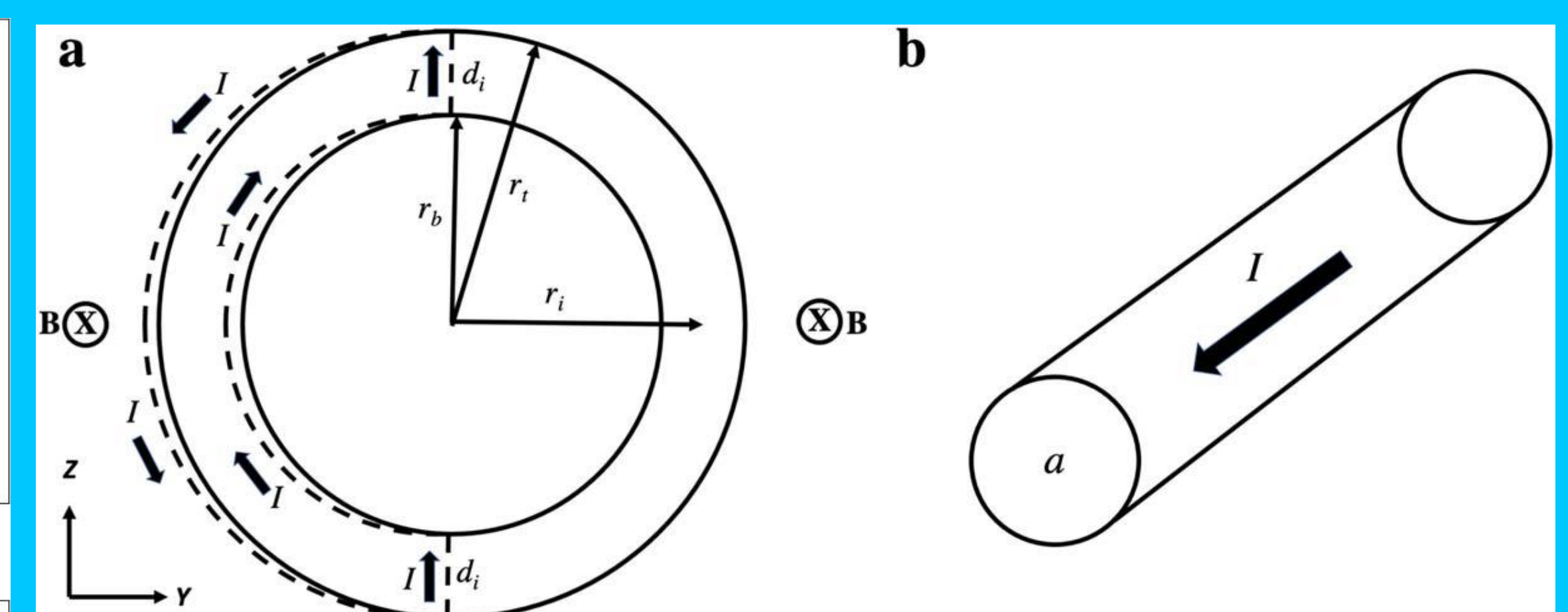
Figure 3. Left: the geometry of the problem. The stellar wind magnetic flux is going through the ionospheric cross section, which is determined by the area bounded between r_b and r_i . The current, I , induced by dB/dt is flowing in a closed loop with an approximated length 2\pi r_i (dashed line) and a cross section, a (shown on the right).
