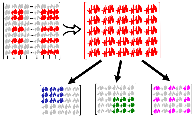
Figure 3 – Systematic Selection of FRF Submatrices for SVD
