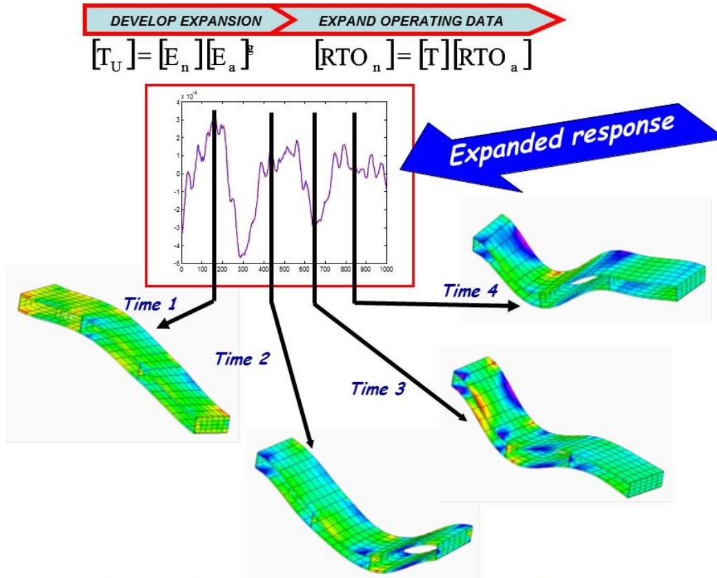
Dynamic stress prediction at various times during transient
